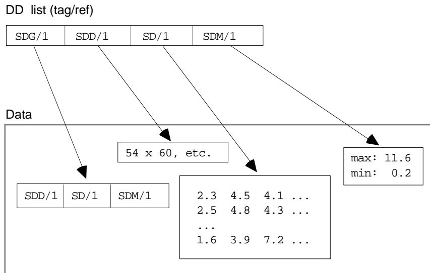
Figure 4.3 SDG Structure
