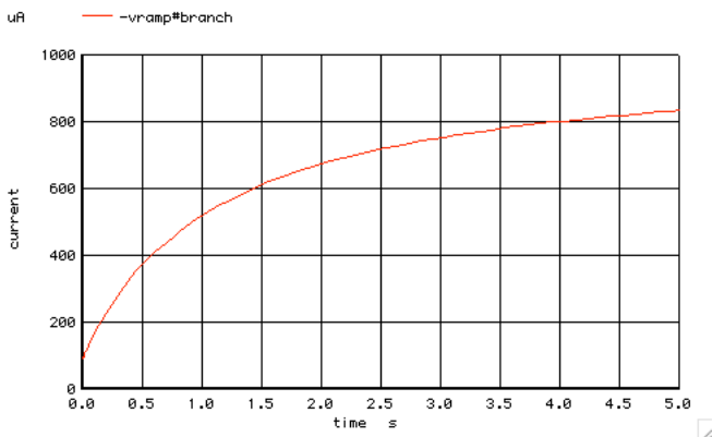
Graph 47 - tran46: PINCH_RESISTOR
